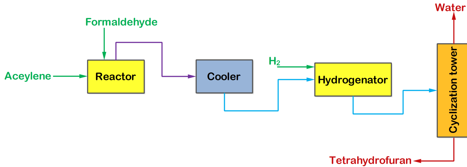
Figure: Manufacture of tetrahydrofuran from acetylene
